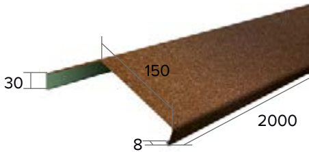
Ridge cap 150
