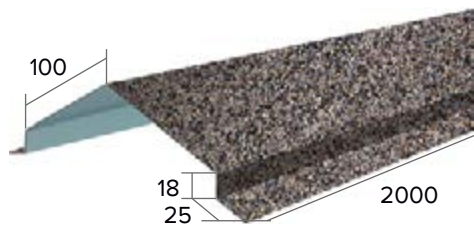
Ridge cap 100
