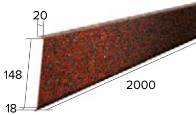
Fascia flashing
