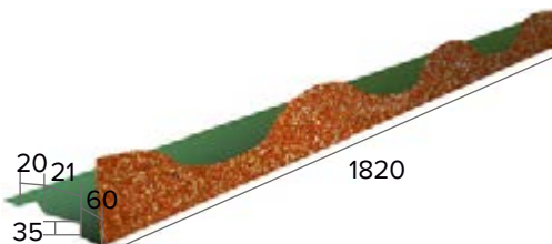
Bird stop
