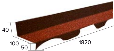
Top course
