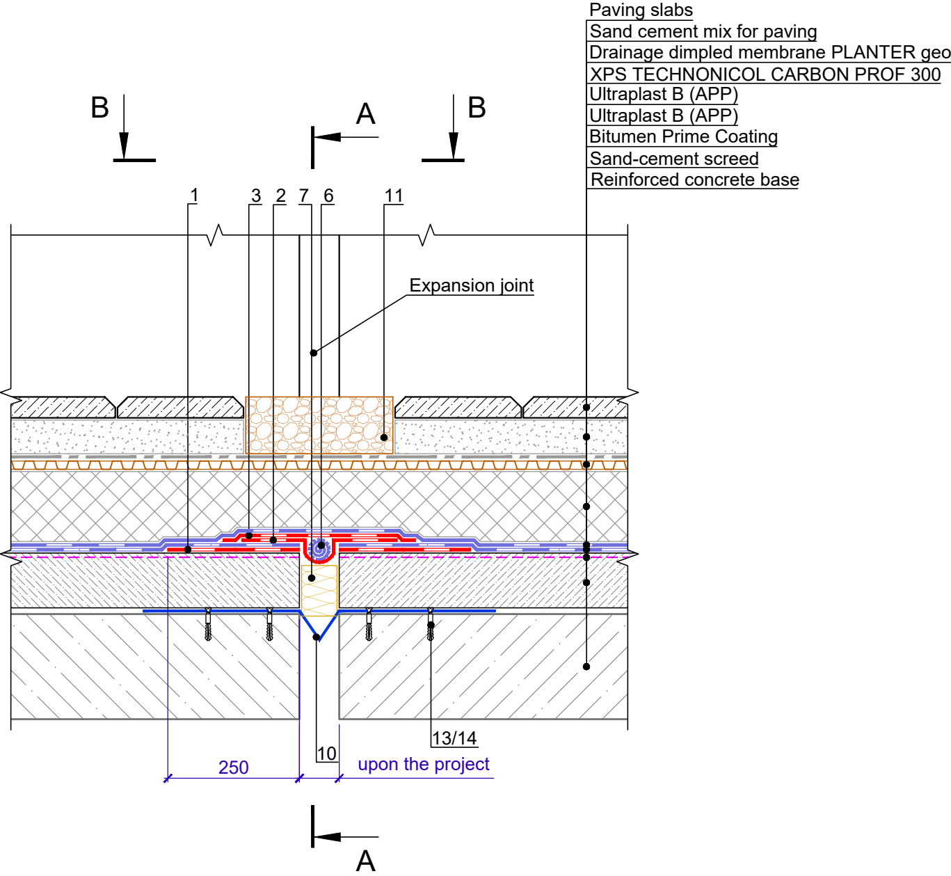
Specification of detail DWG No. 6.2 - 2021.04
