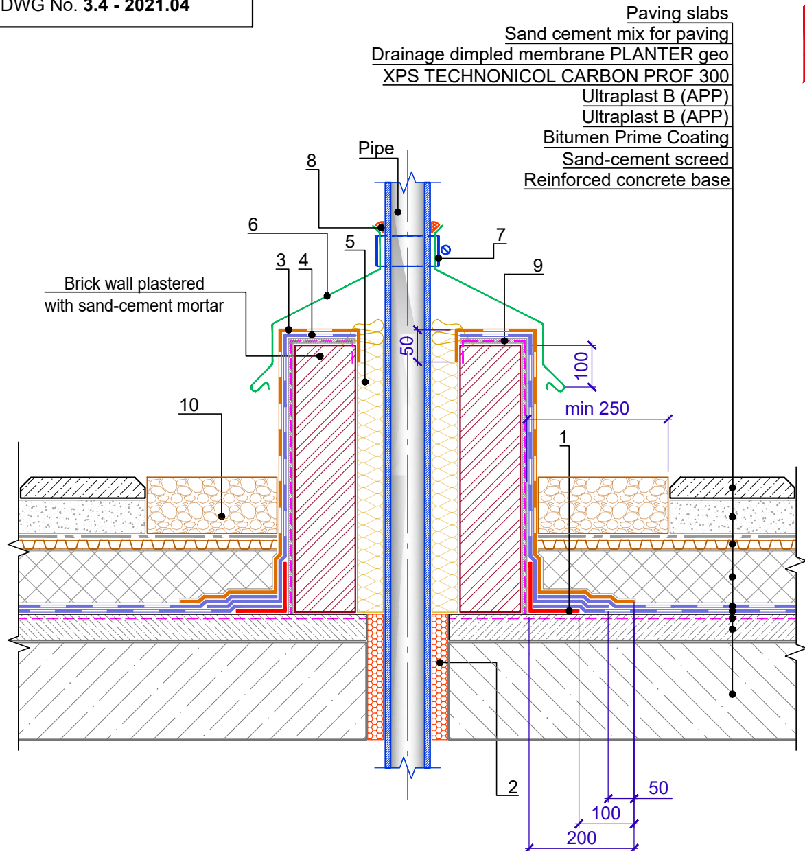
Specification of detail DWG No. 3.4 - 2021.04
