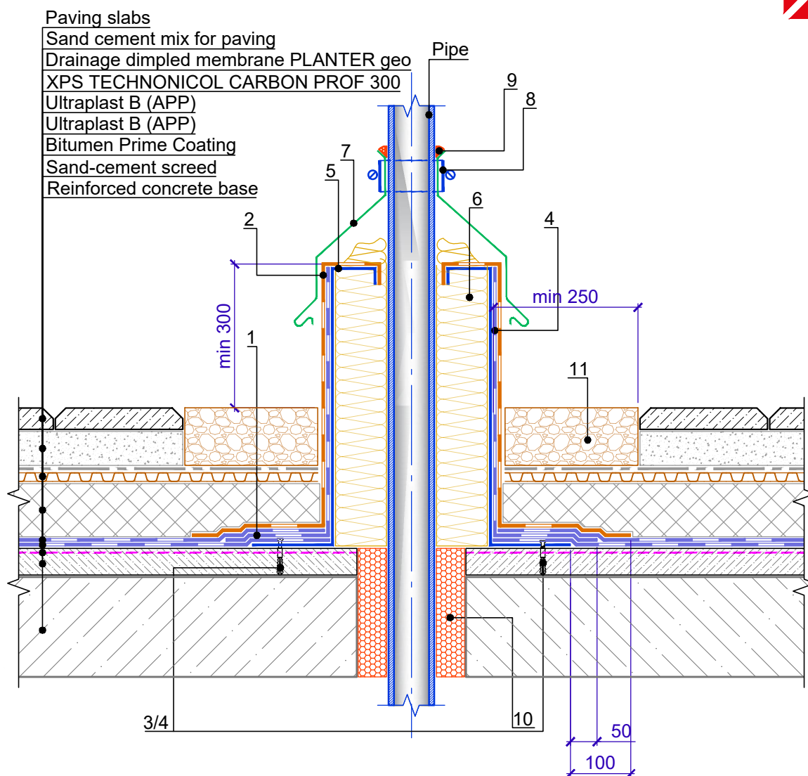
Specification of detail DWG No. 3.3 - 2021.04
