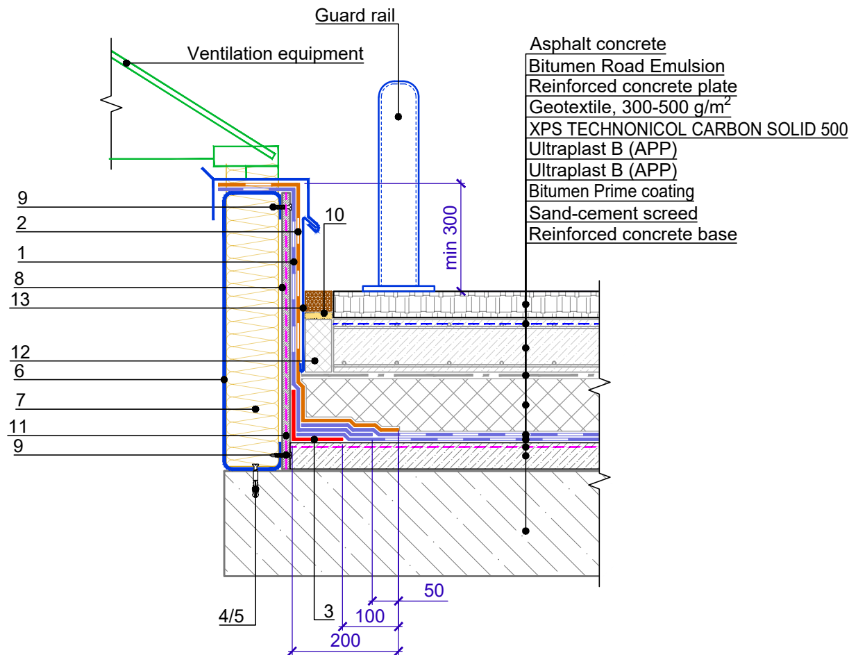
Specification of detail DWG No. 3.1 - 2021.05
