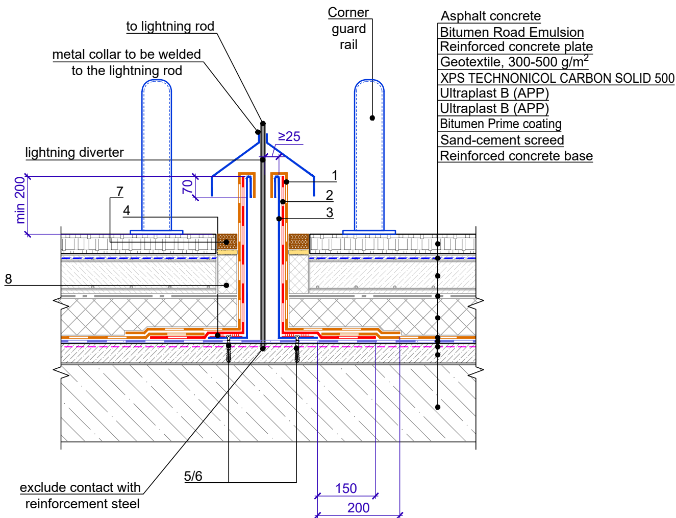
Specification of detail DWG No. 8.2 - 2021.05
