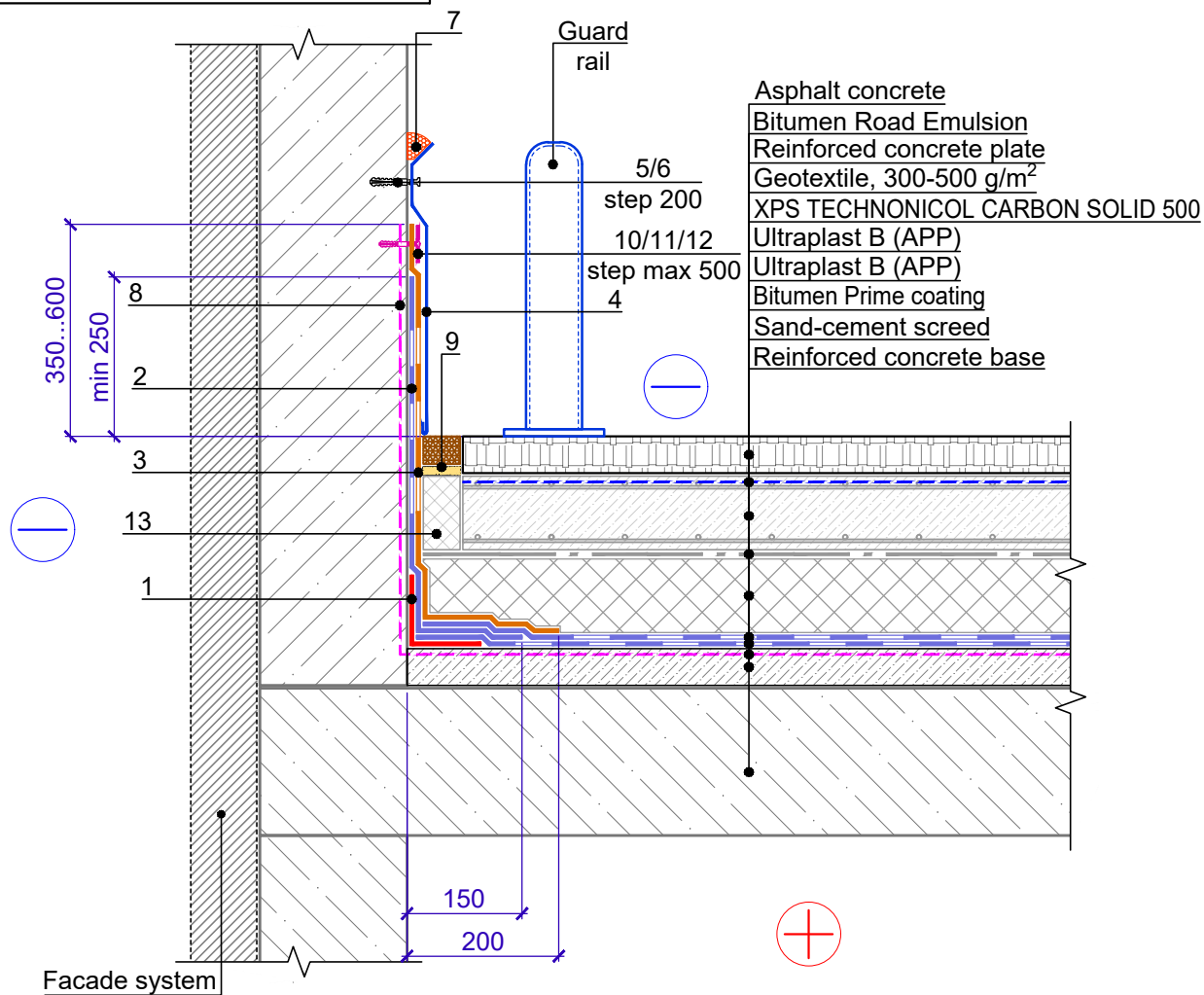
Specification of detail DWG No. 2.1 - 2021.05
