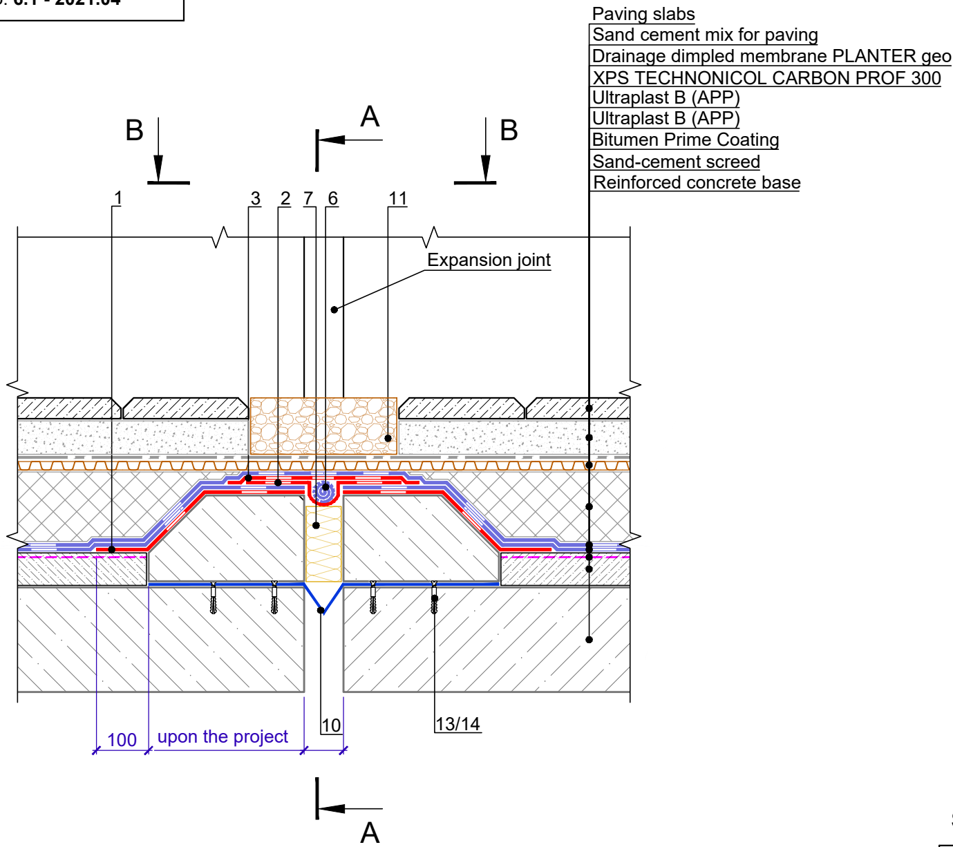
Specification of detail DWG No. 6.1 - 2021.04
