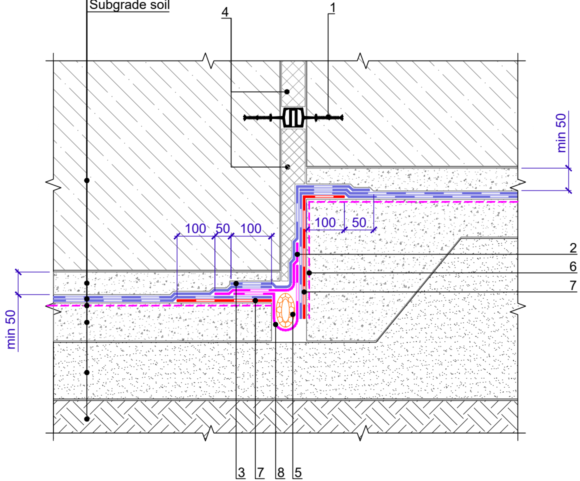
Specification of detail DWG No. 3.5 - 2021.07
