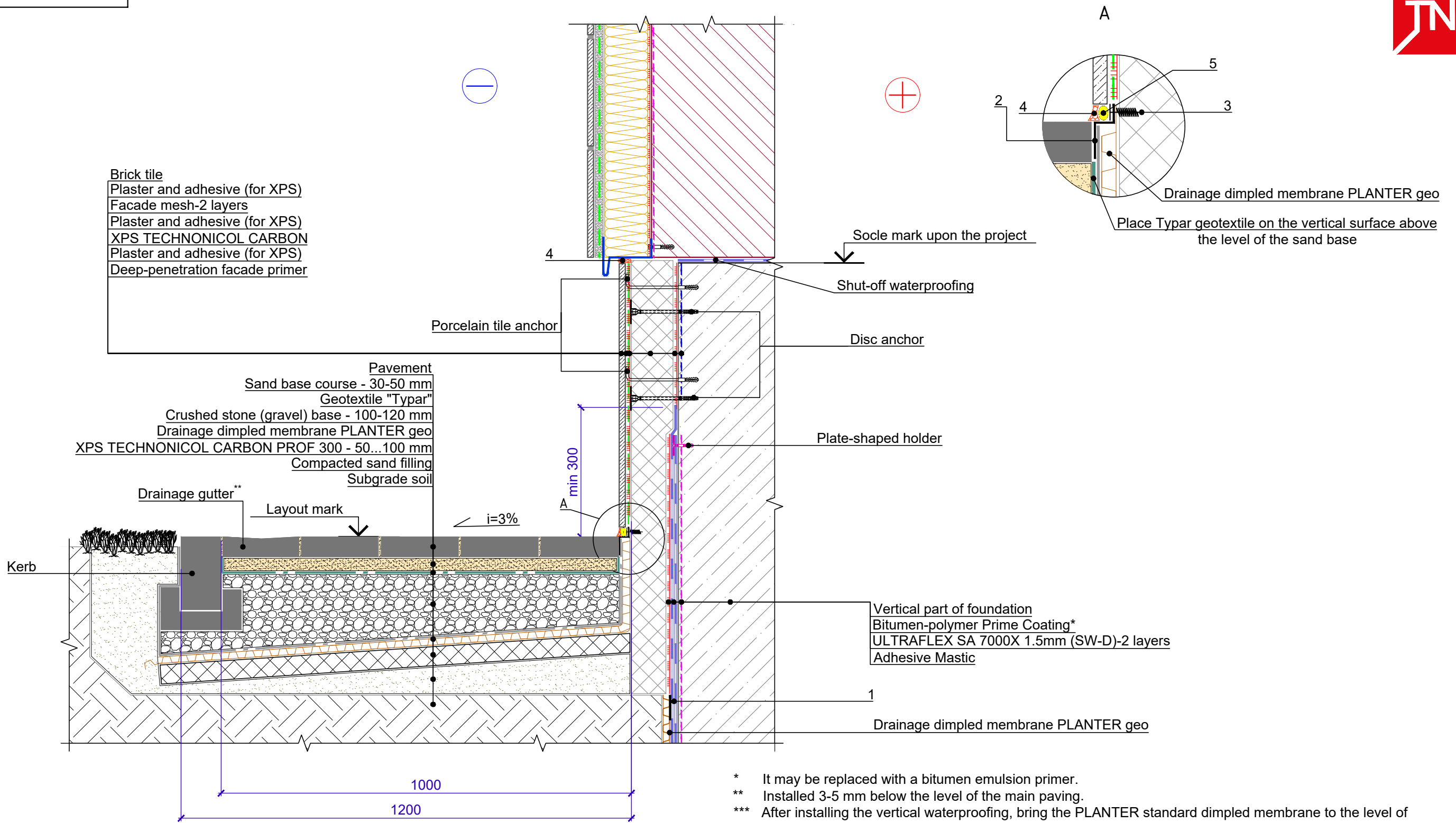
Specification of detail DWG No. 4.1 - 2021.07
